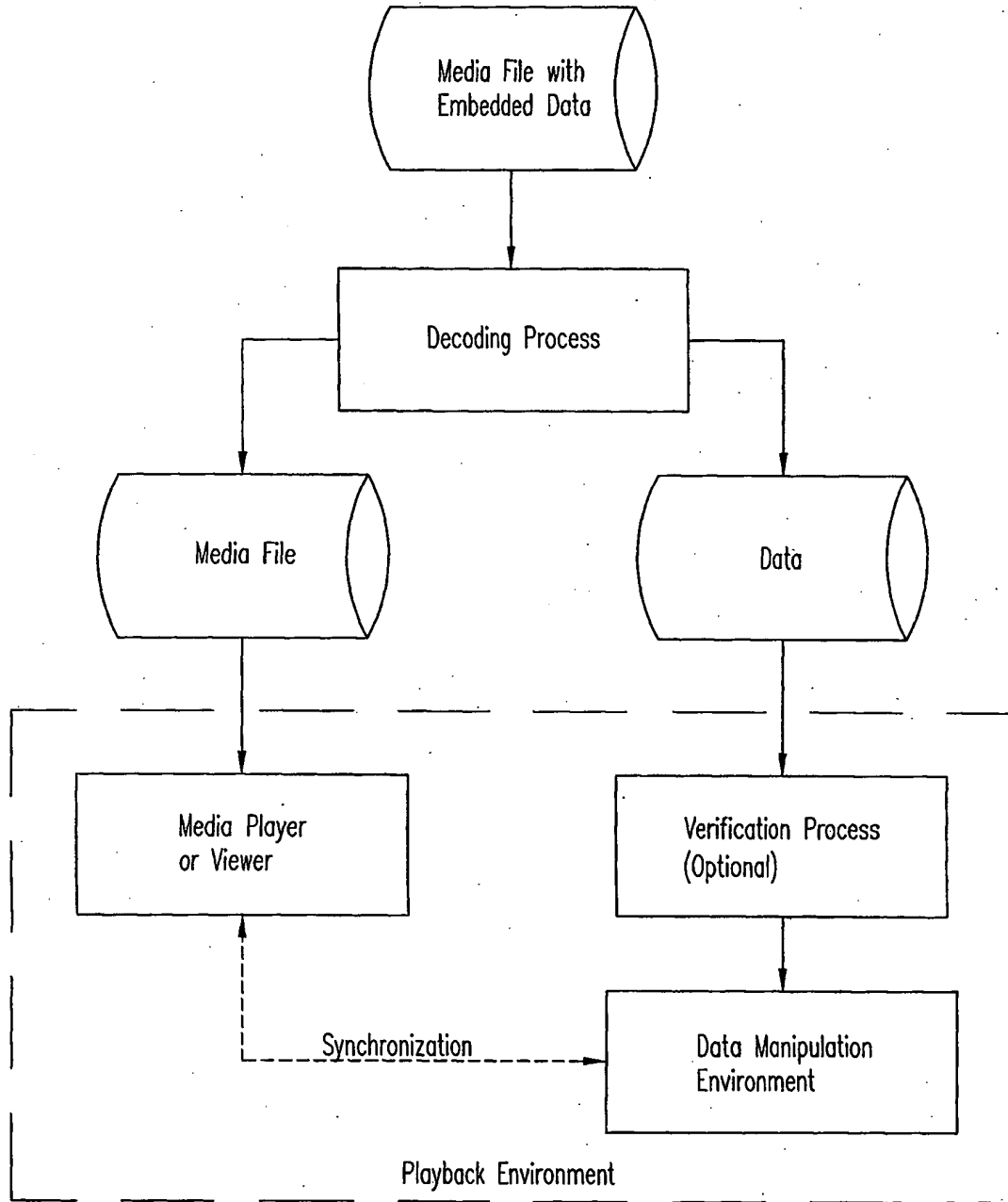
Data Encoding Playback Overview
